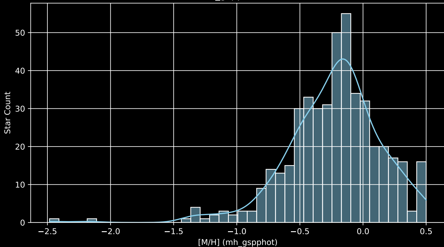
APOGEE DR17 Field: [200+45 [M/H] (mh_gspphot) (n= 459)
