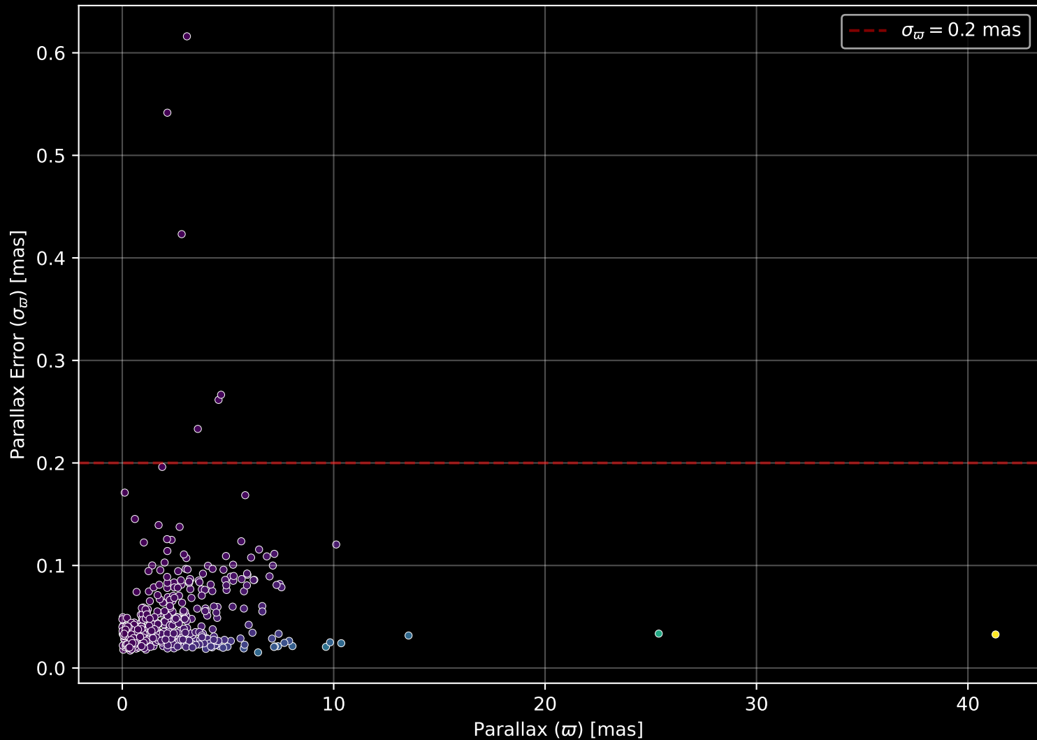
APOGEE DR17 Field: [200+45] Parallax Quality (n= 463)
