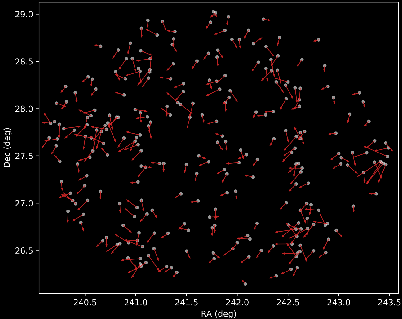
APOGEE DR17 Cluster 6 Proper Motion Vectors (n=268)
