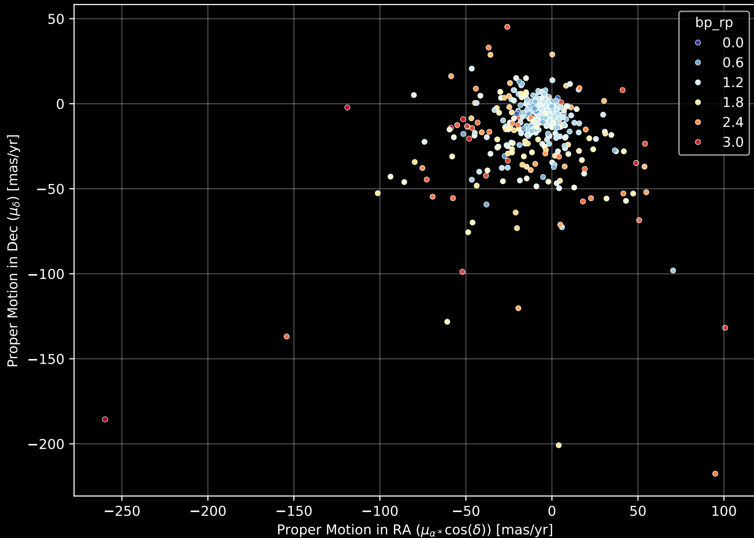
APOGEE DR17 Field: [200+45] Proper Motion Diagram (n= 463)
