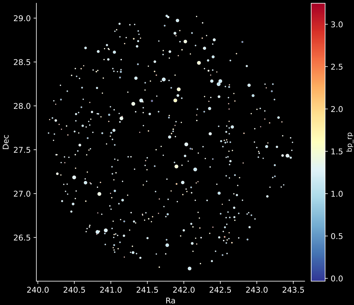
APOGEE DR17 Field: [200+45] Stars: 463
