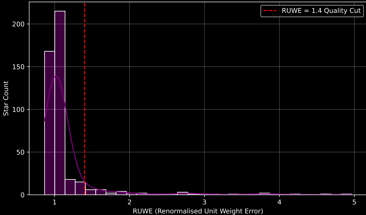
GAPOGEE DR17 Field [200+45] RUWE Distribution (n= 454)
